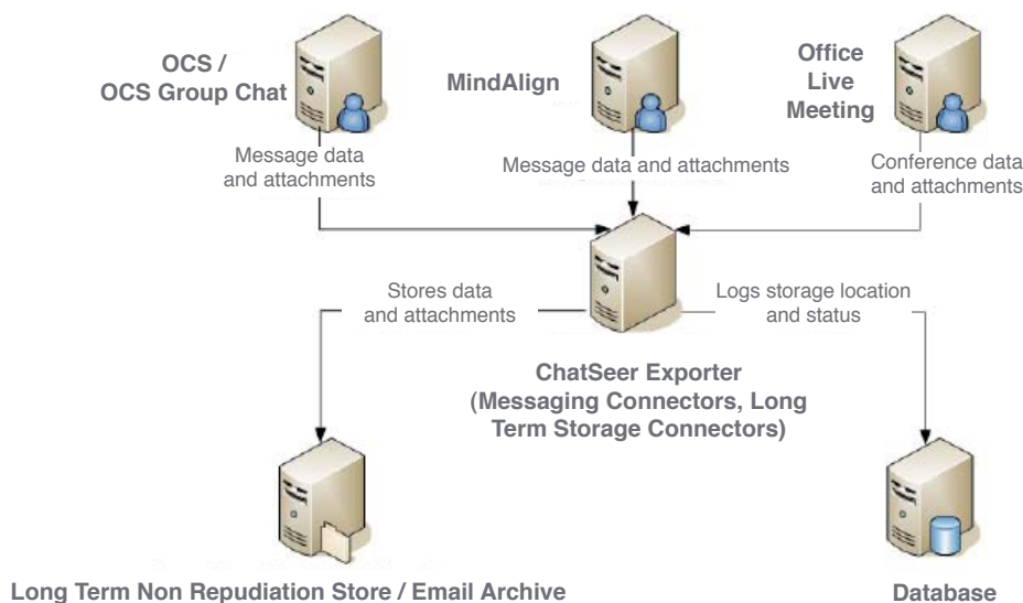
System workflow of ChatSeer Exporter
